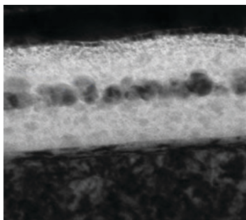
Actual cross section of HyProtect coating
